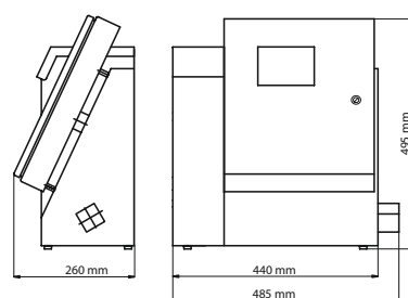
Machine (22 kg)
