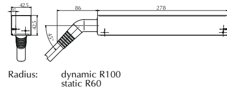
Print head (ca. 1 kg)
